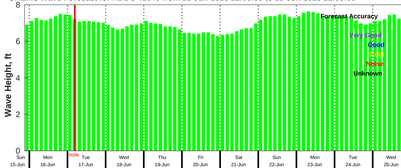
CMEMS Wave Forecast for NDBC 41040 from 15-Jun-2025 21:00:00 to 25-Jun-2025 21:00:00
