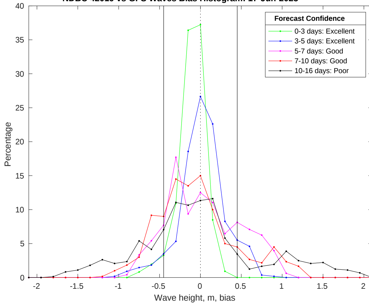
NDBC 42019 vs GFS Waves Bias Histogram: 17-Jun-2025
