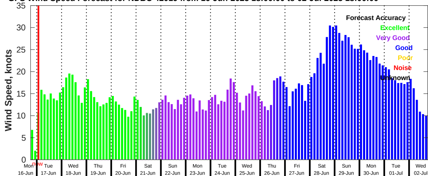
GFS Wind Speed Forecast for NDBC 42019 from 16-Jun-2025 18:00:00 to 02-Jul-2025 18:00:00
