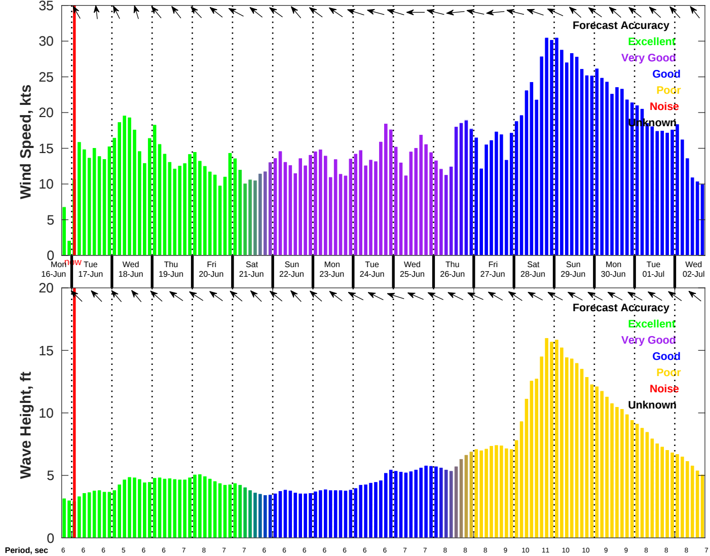
Wind & Wave Forecast for NDBC 42019 from 16-Jun-2025 18:00:00 to 02-Jul-2025 18:00:00
