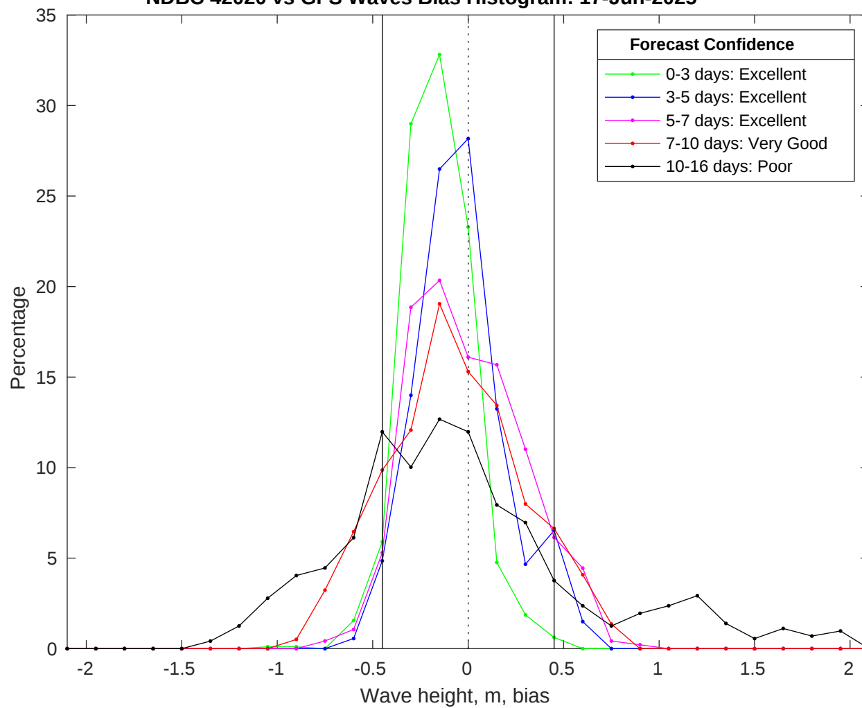
NDBC 42020 vs GFS Waves Bias Histogram: 17-Jun-2025
