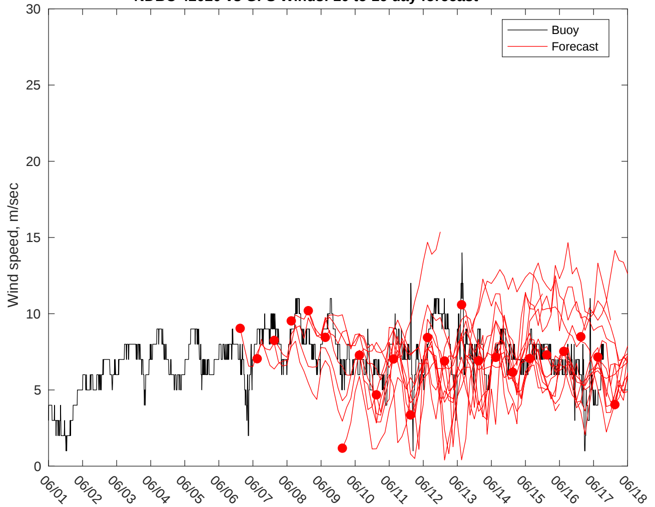
NDBC 42020 vs GFS Winds: 10 to 16 day forecast
