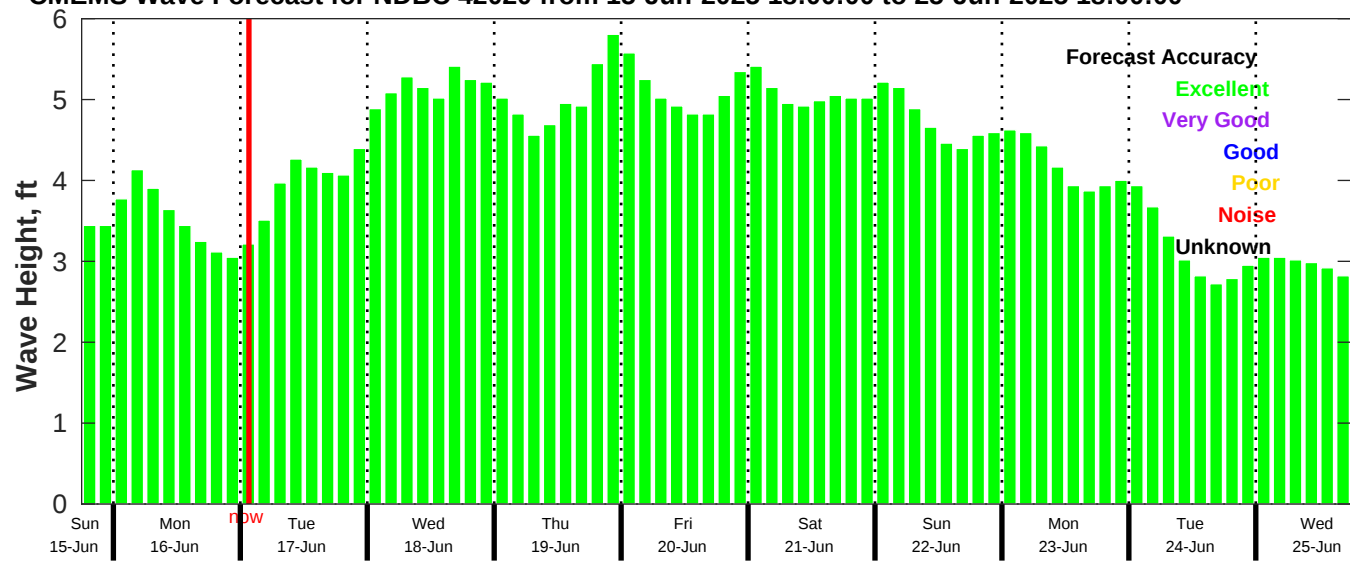
CMEMS Wave Forecast for NDBC 42020 from 15-Jun-2025 18:00:00 to 25-Jun-2025 18:00:00
