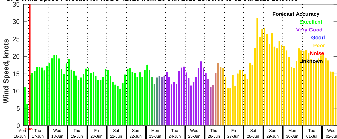
GFS Wind Speed Forecast for NDBC 42020 from 16-Jun-2025 18:00:00 to 02-Jul-2025 18:00:00
