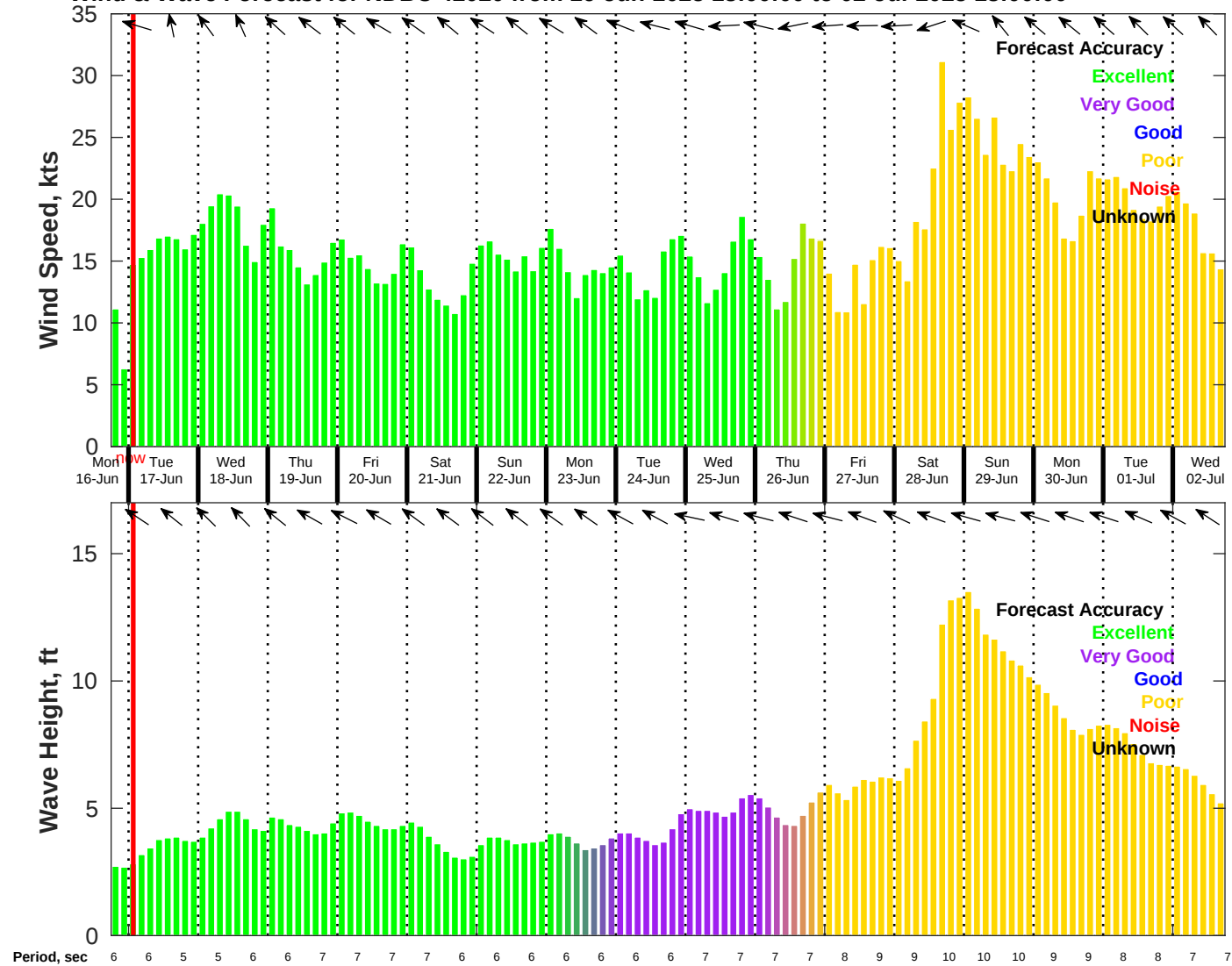
Wind & Wave Forecast for NDBC 42020 from 16-Jun-2025 18:00:00 to 02-Jul-2025 18:00:00
