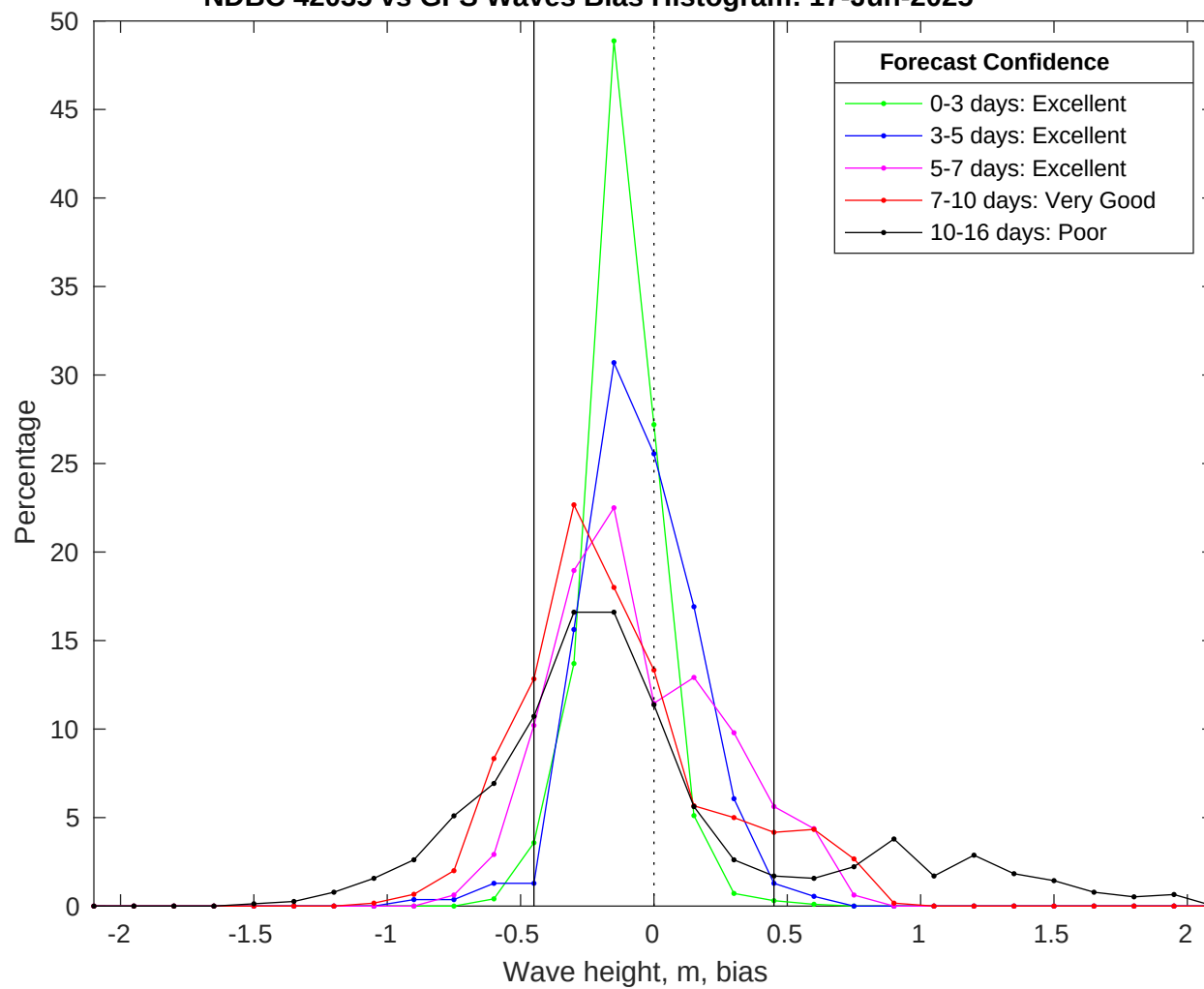
NDBC 42035 vs GFS Waves Bias Histogram: 17-Jun-2025
