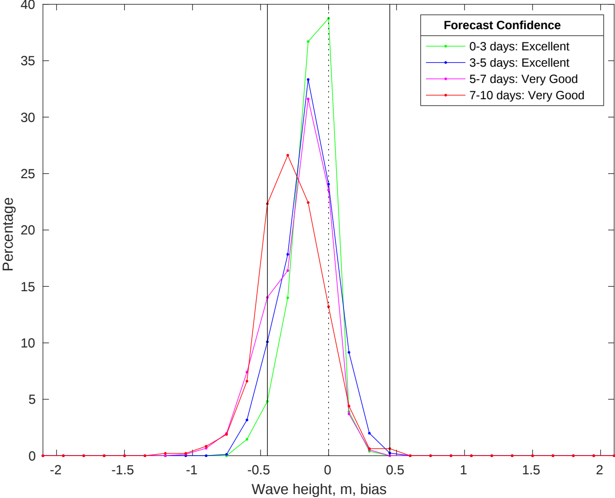
NDBC 42036 vs CMEMS Waves Bias Histogram: 17-Jun-2025
