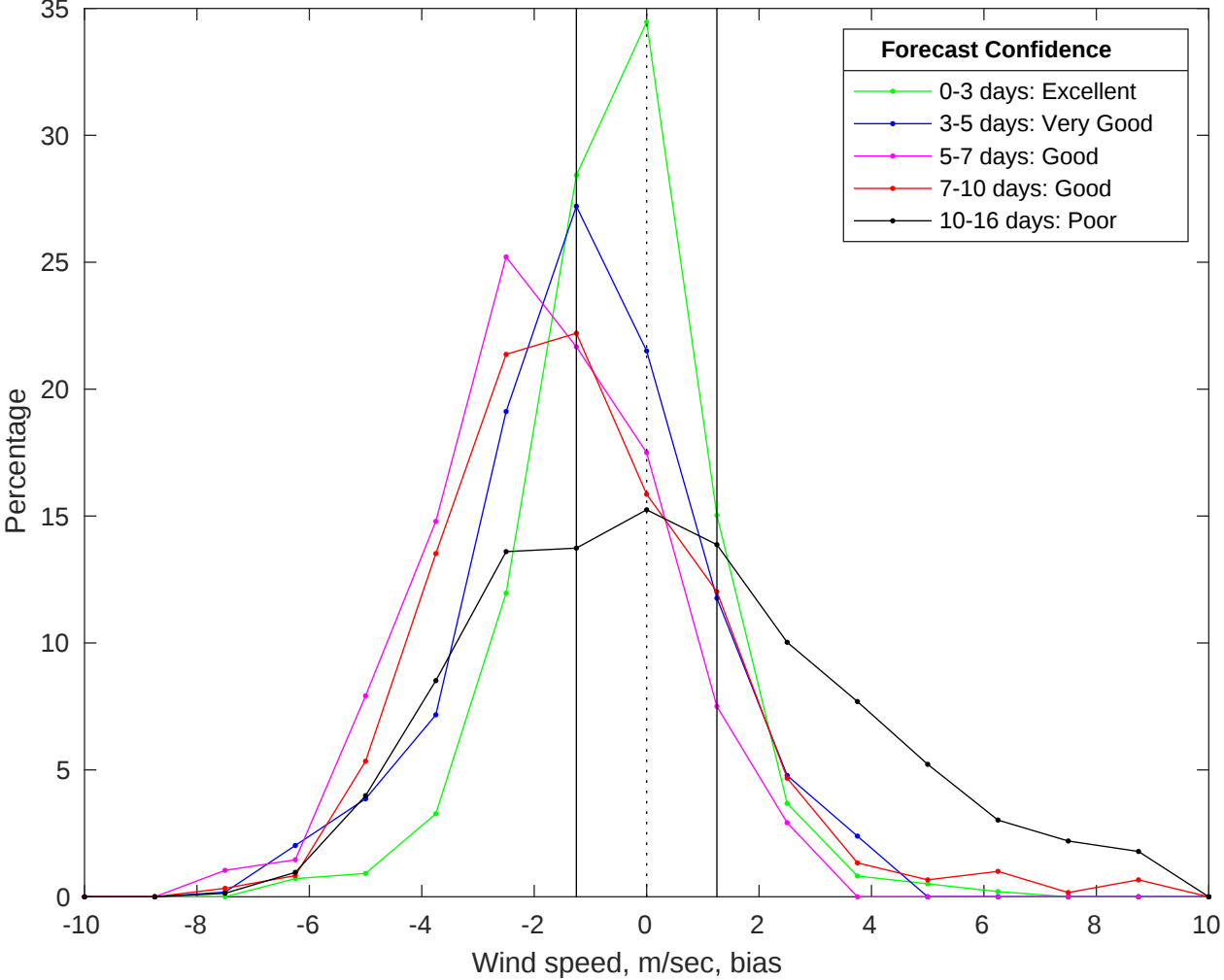
NDBC 42036 vs GFS Winds Bias Histogram: 17-Jun-2025
