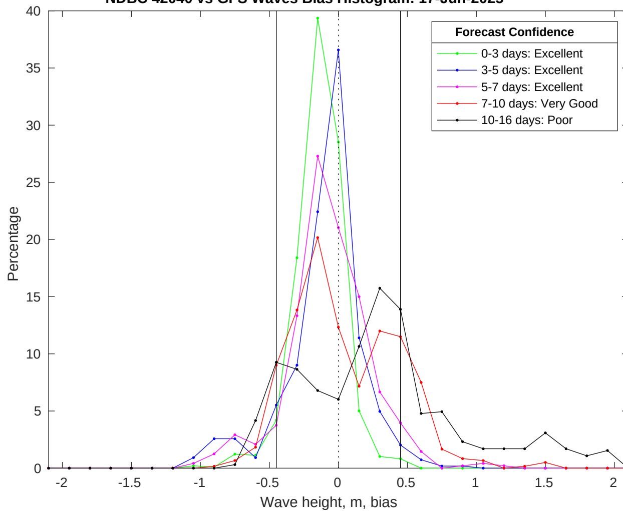
NDBC 42040 vs GFS Waves Bias Histogram: 17-Jun-2025
