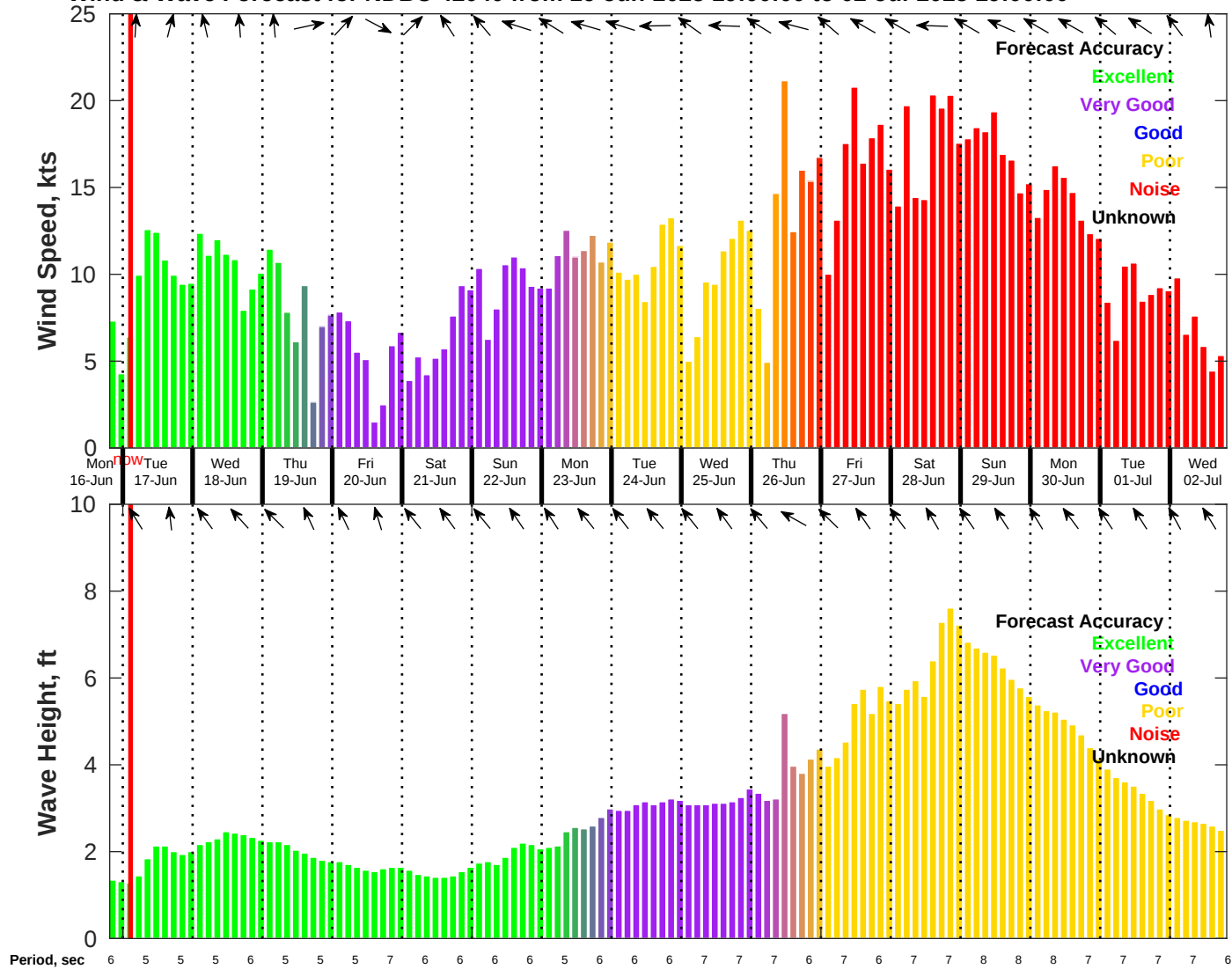
Wind & Wave Forecast for NDBC 42040 from 16-Jun-2025 19:00:00 to 02-Jul-2025 19:00:00
