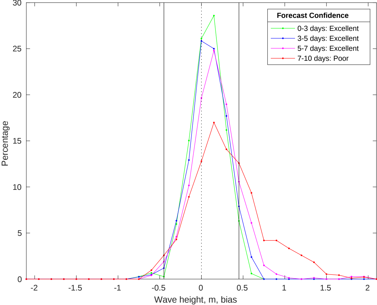
NDBC 46011 vs CMEMS Waves Bias Histogram: 17-Jun-2025
