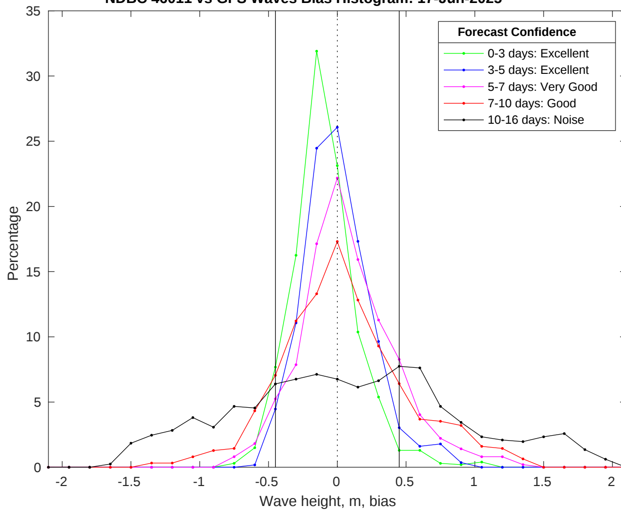
NDBC 46011 vs GFS Waves Bias Histogram: 17-Jun-2025
