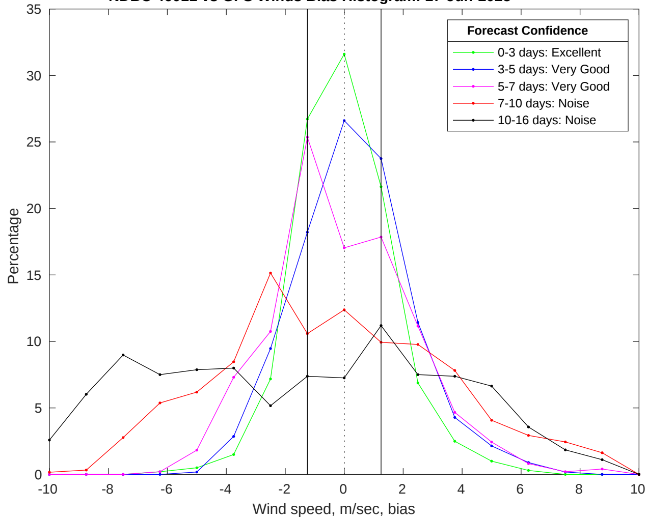
NDBC 46011 vs GFS Winds Bias Histogram: 17-Jun-2025
