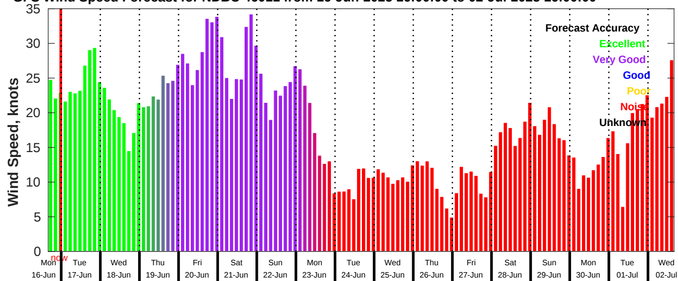
GFS Wind Speed Forecast for NDBC 46011 from 16-Jun-2025 16:00:00 to 02-Jul-2025 16:00:00
