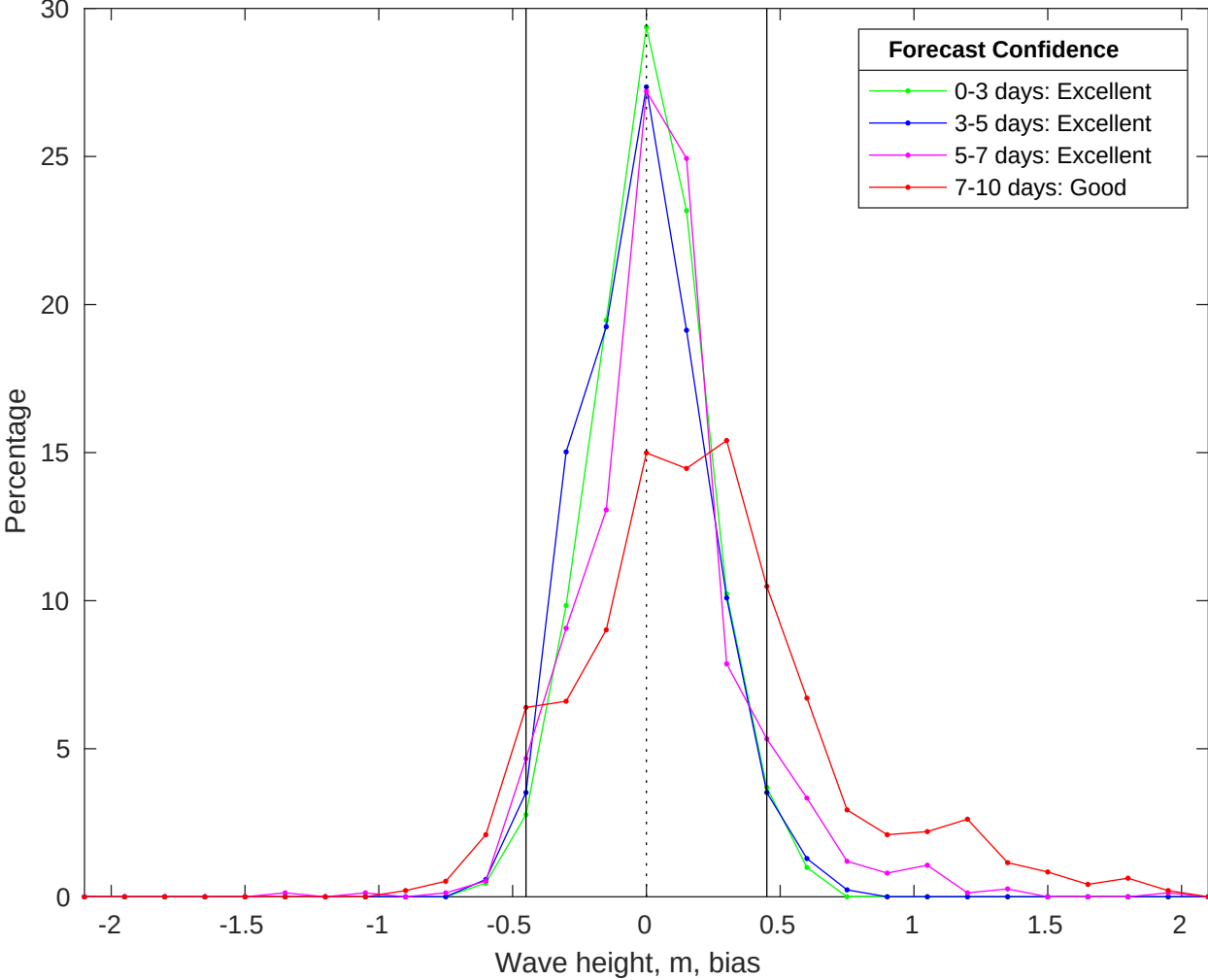
NDBC 46028 vs CMEMS Waves Bias Histogram: 17-Jun-2025
