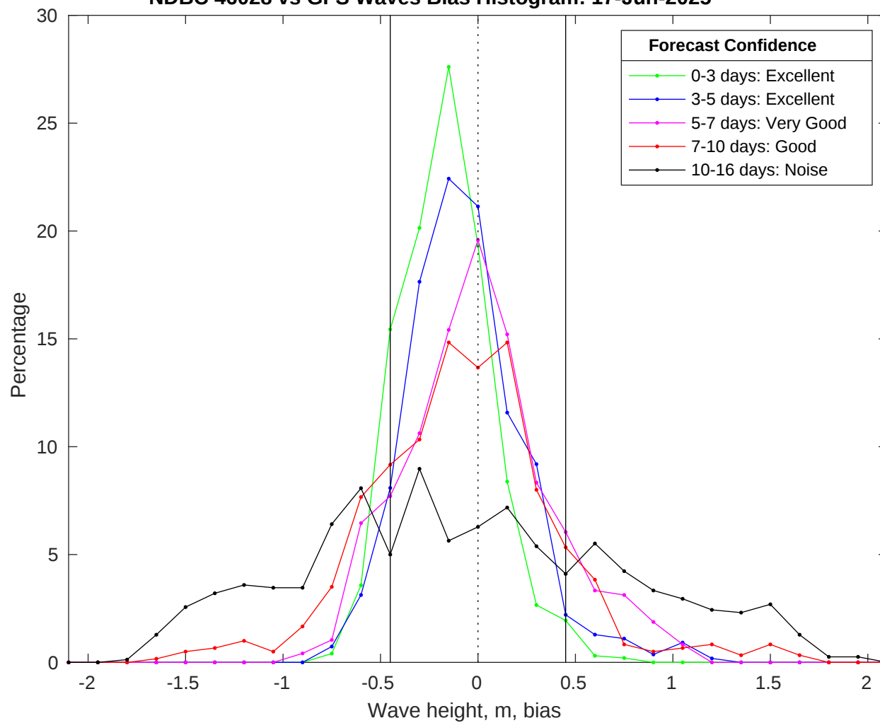
NDBC 46028 vs GFS Waves Bias Histogram: 17-Jun-2025
