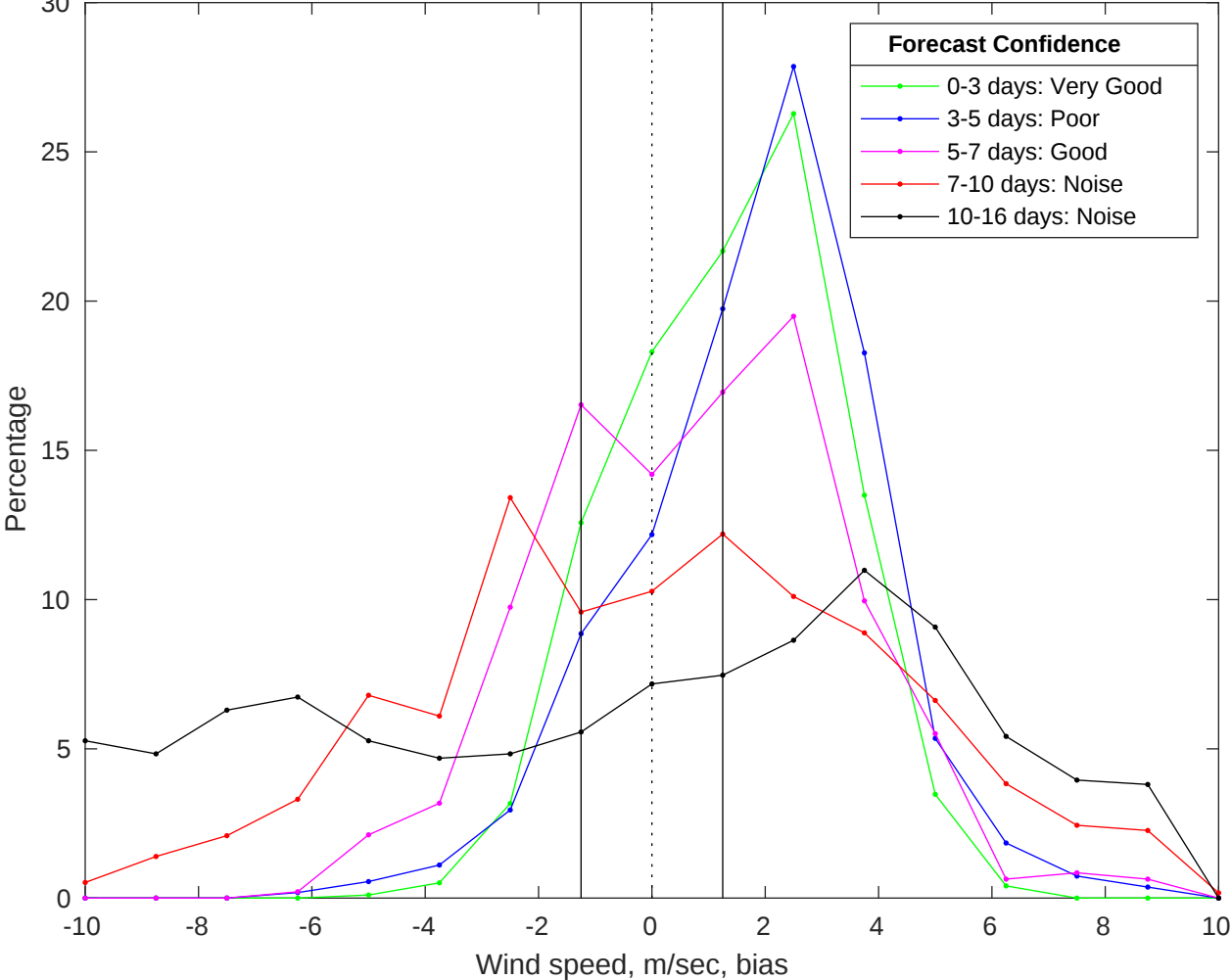
NDBC 46028 vs GFS Winds Bias Histogram: 17-Jun-2025
