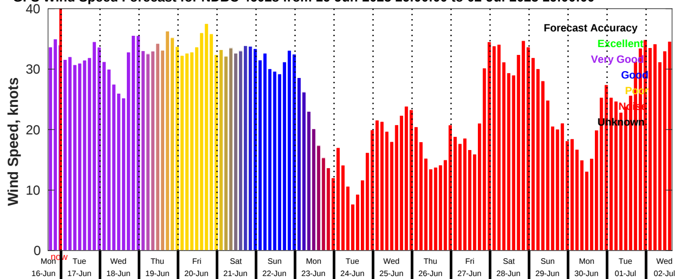
GFS Wind Speed Forecast for NDBC 46028 from 16-Jun-2025 16:00:00 to 02-Jul-2025 16:00:00
