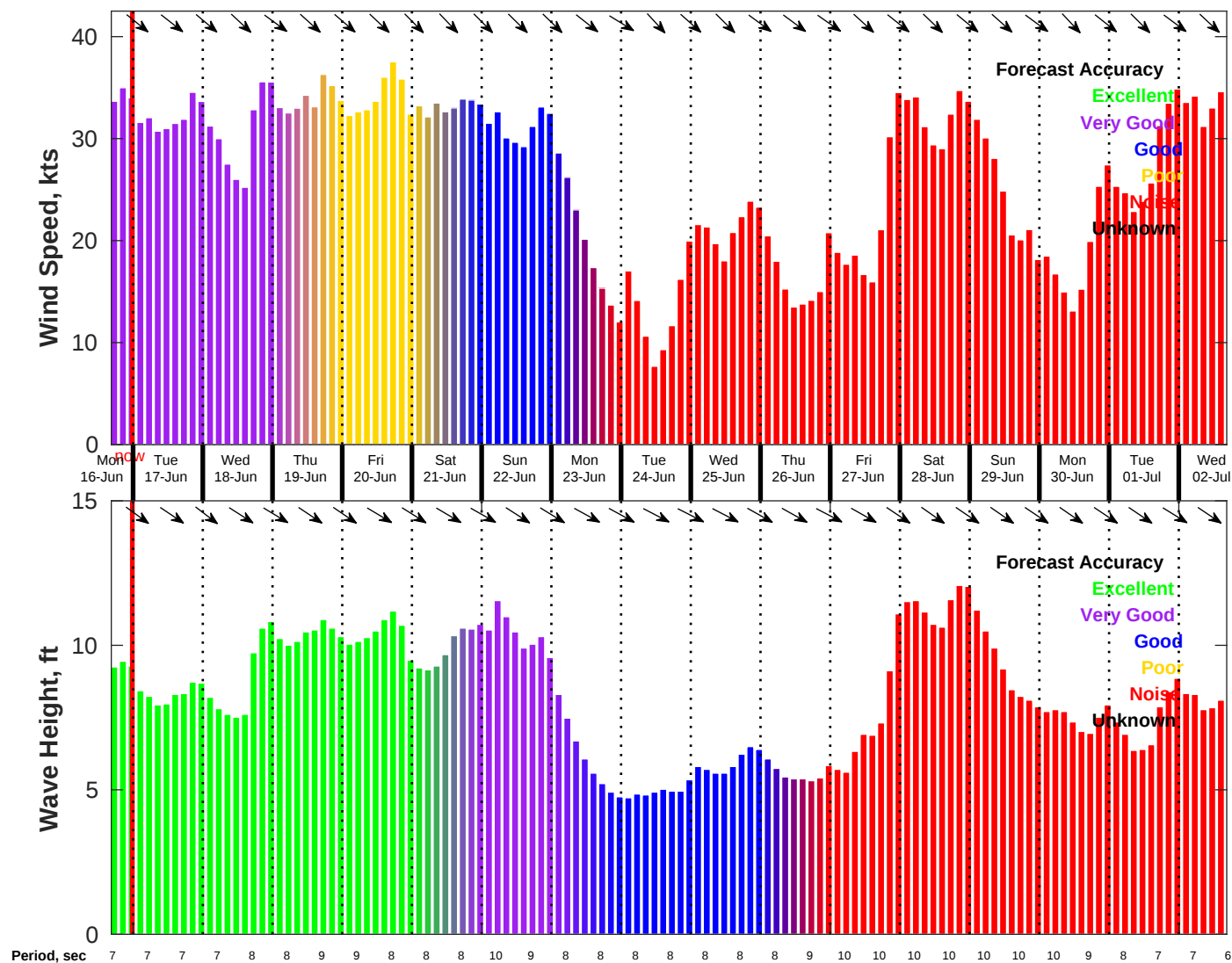
Wind & Wave Forecast for NDBC 46028 from 16-Jun-2025 16:00:00 to 02-Jul-2025 16:00:00
