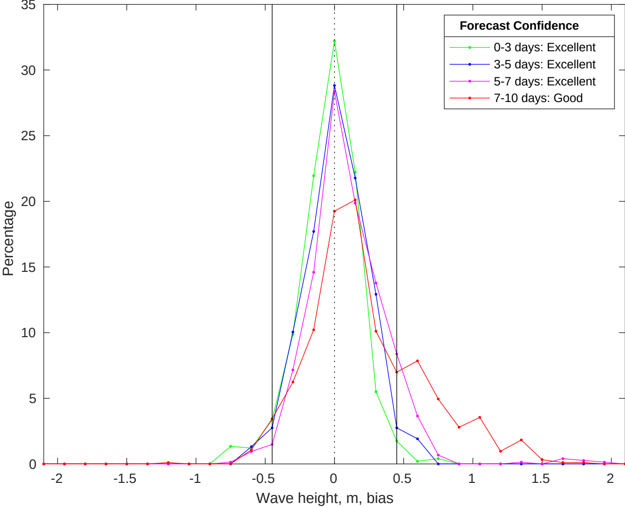
NDBC 46054 vs CMEMS Waves Bias Histogram: 17-Jun-2025
