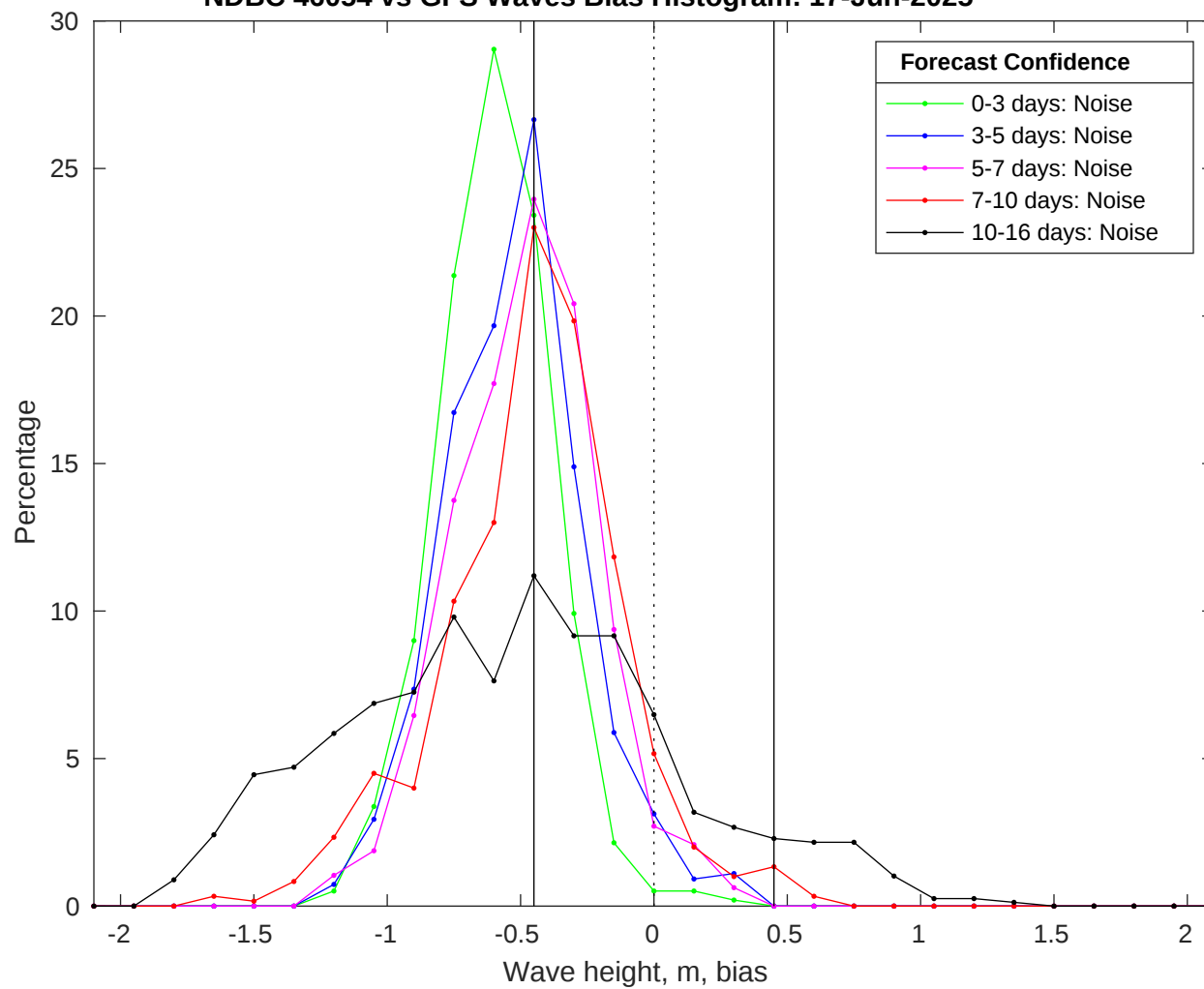
NDBC 46054 vs GFS Waves Bias Histogram: 17-Jun-2025
