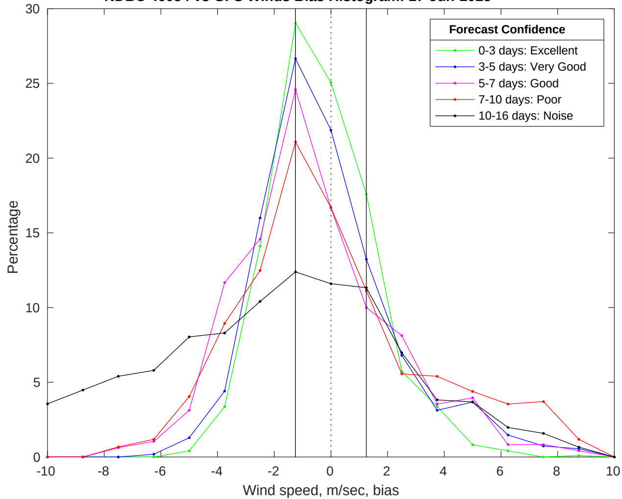
NDBC 46054 vs GFS Winds Bias Histogram: 17-Jun-2025
