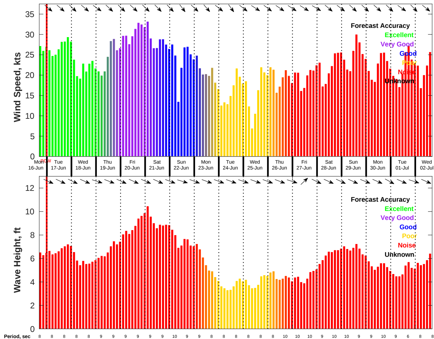
Wind & Wave Forecast for NDBC 46054 from 16-Jun-2025 16:00:00 to 02-Jul-2025 16:00:00
