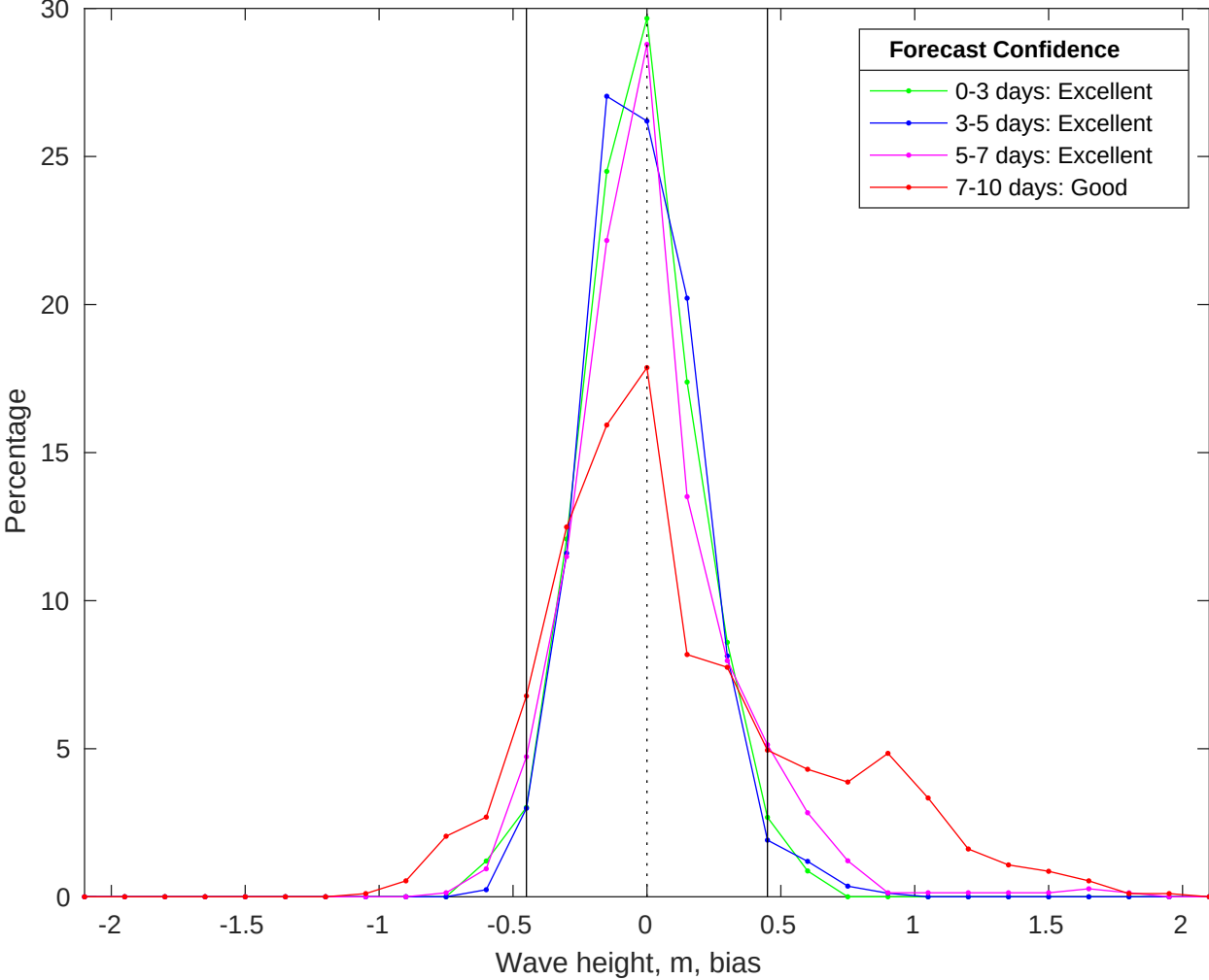
NDBC 46069 vs CMEMS Waves Bias Histogram: 17-Jun-2025
