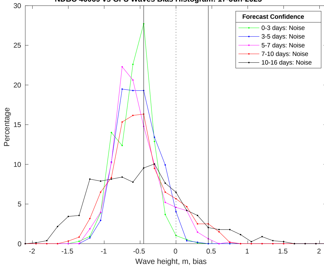
NDBC 46069 vs GFS Waves Bias Histogram: 17-Jun-2025
