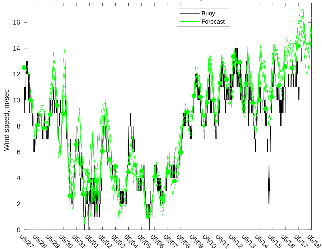
NDBC 46069 vs GFS Winds: 0 to 3 day forecast
