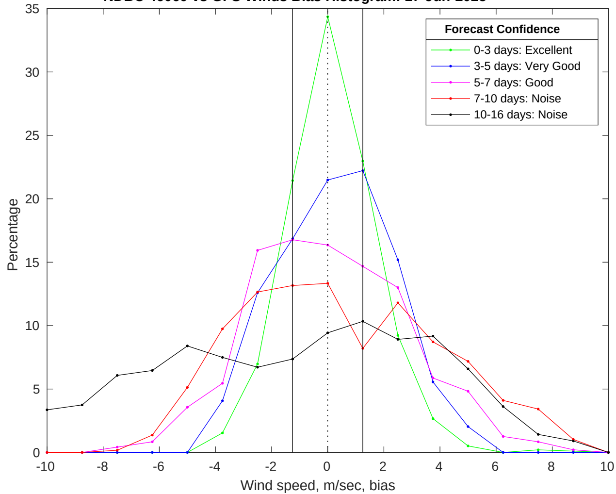
NDBC 46069 vs GFS Winds Bias Histogram: 17-Jun-2025
