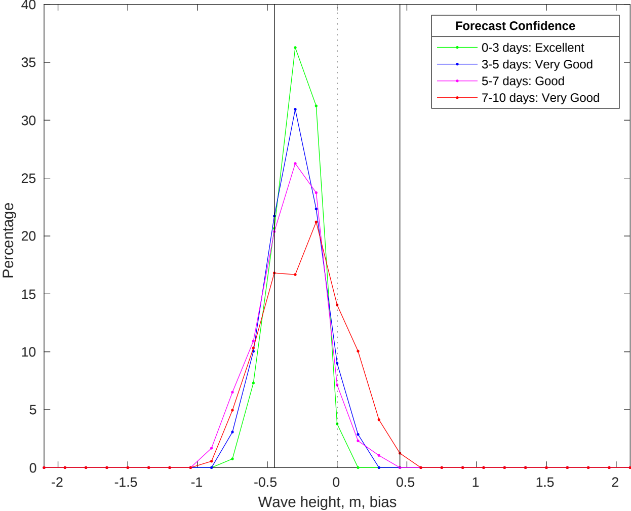
NDBC 51209 vs CMEMS Waves Bias Histogram: 17-Jun-2025
