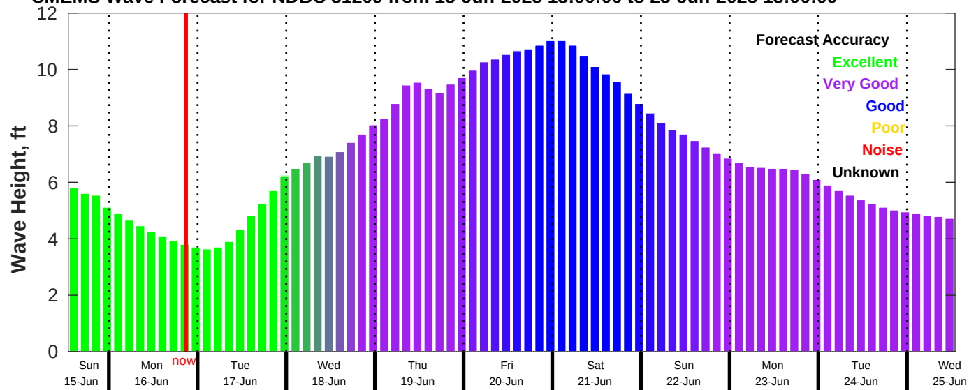
CMEMS Wave Forecast for NDBC 51209 from 15-Jun-2025 13:00:00 to 25-Jun-2025 13:00:00
