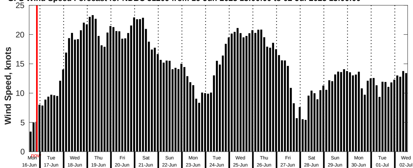
GFS Wind Speed Forecast for NDBC 51209 from 16-Jun-2025 13:00:00 to 02-Jul-2025 13:00:00
