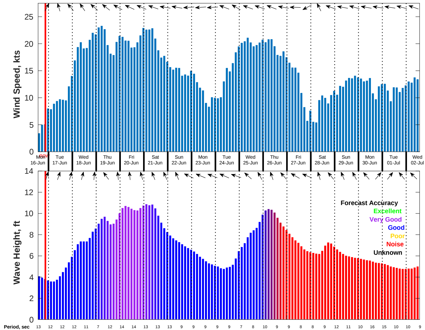
Wind & Wave Forecast for NDBC 51209 from 16-Jun-2025 13:00:00 to 02-Jul-2025 13:00:00
