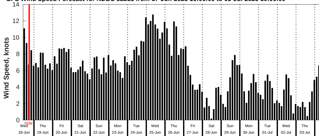
GFS Wind Speed Forecast for NDBC 52211 from 17-Jun-2025 10:00:00 to 03-Jul-2025 10:00:00
