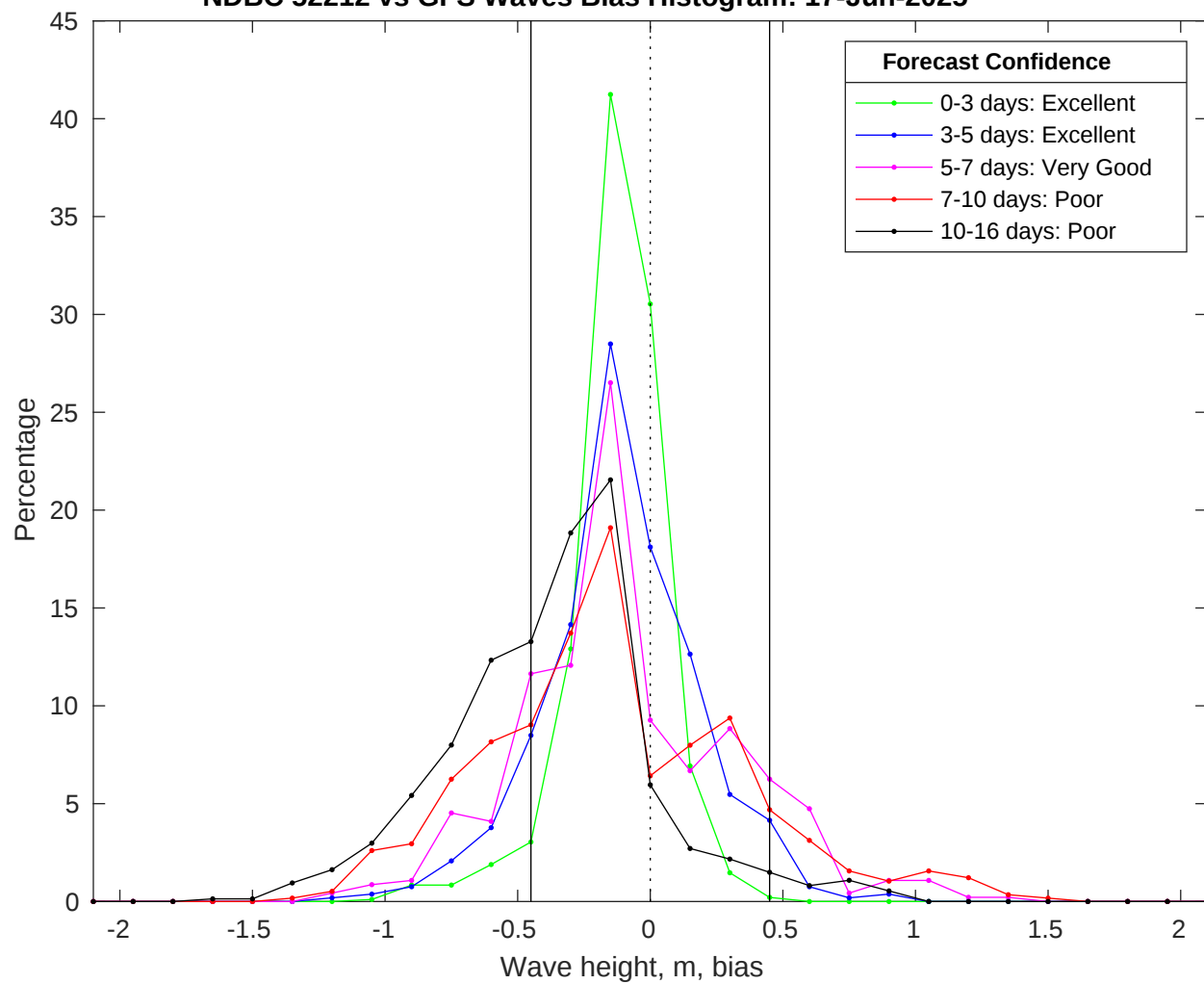
NDBC 52212 vs GFS Waves Bias Histogram: 17-Jun-2025
