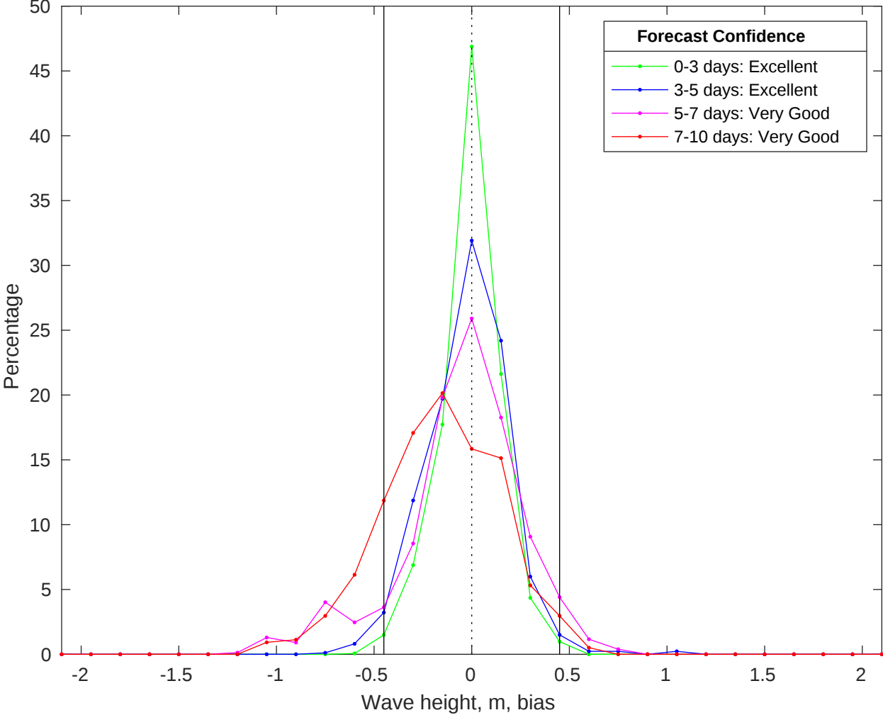
NDBC 41004 vs CMEMS Waves Bias Histogram: 18-Jun-2025
