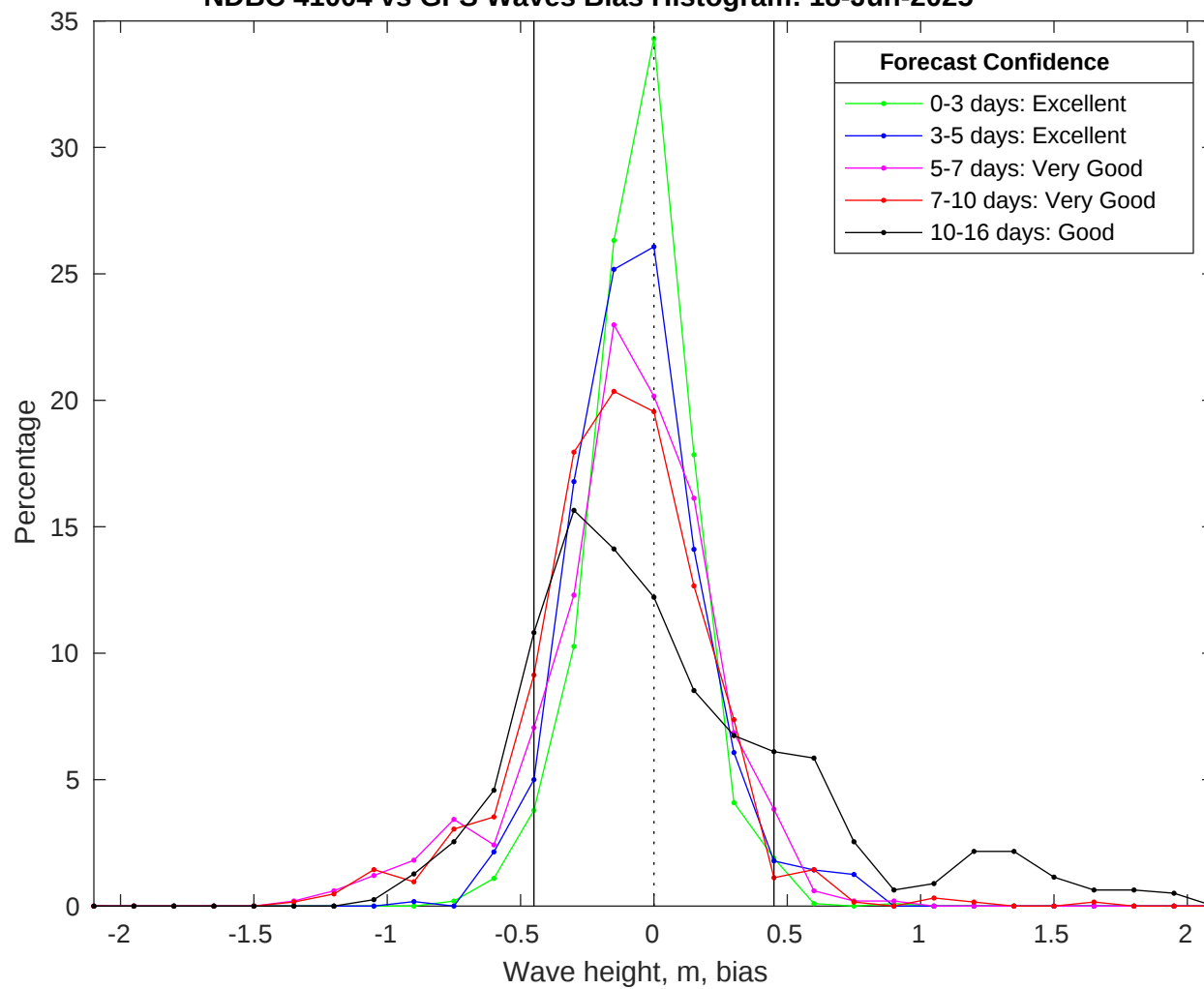
NDBC 41004 vs GFS Waves Bias Histogram: 18-Jun-2025
