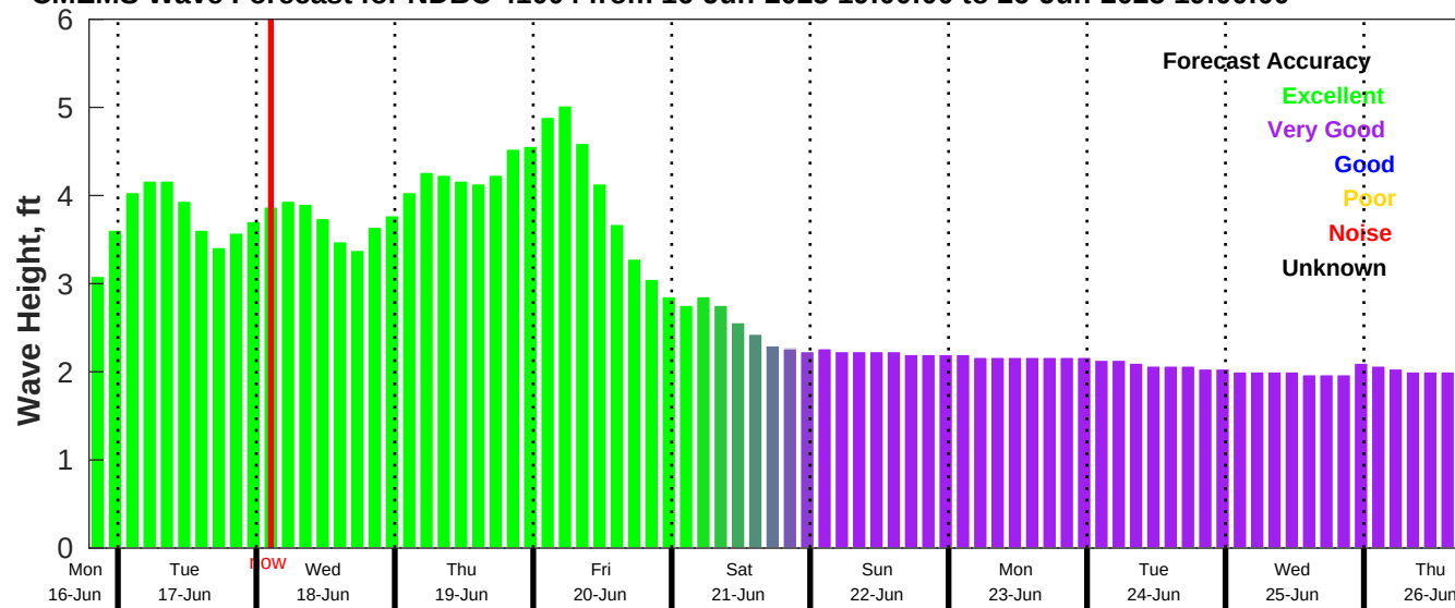
CMEMS Wave Forecast for NDBC 41004 from 16-Jun-2025 19:00:00 to 26-Jun-2025 19:00:00
