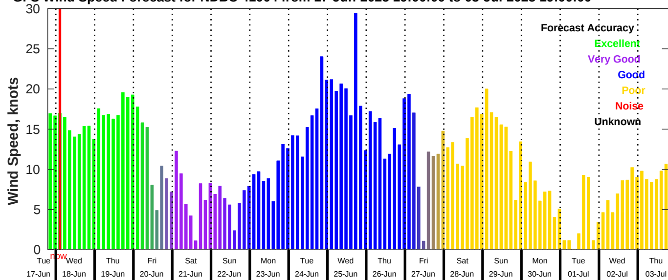
GFS Wind Speed Forecast for NDBC 41004 from 17-Jun-2025 19:00:00 to 03-Jul-2025 19:00:00
