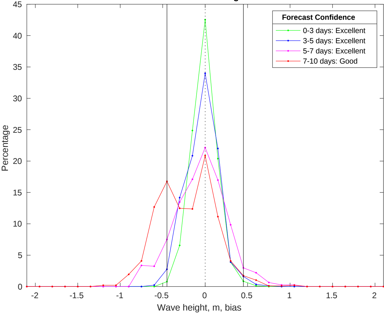
NDBC 41013 vs CMEMS Waves Bias Histogram: 18-Jun-2025
