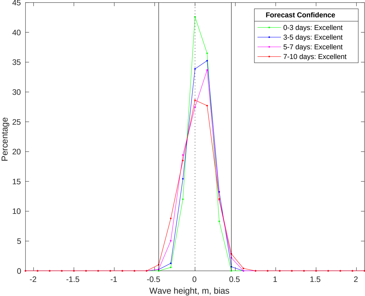
NDBC 41040 vs CMEMS Waves Bias Histogram: 18-Jun-2025
