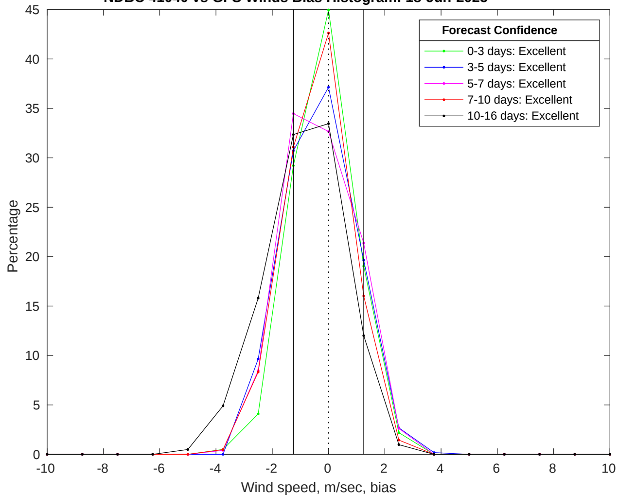
NDBC 41040 vs GFS Winds Bias Histogram: 18-Jun-2025
