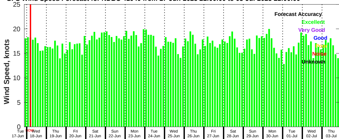
GFS Wind Speed Forecast for NDBC 41040 from 17-Jun-2025 21:00:00 to 03-Jul-2025 21:00:00
