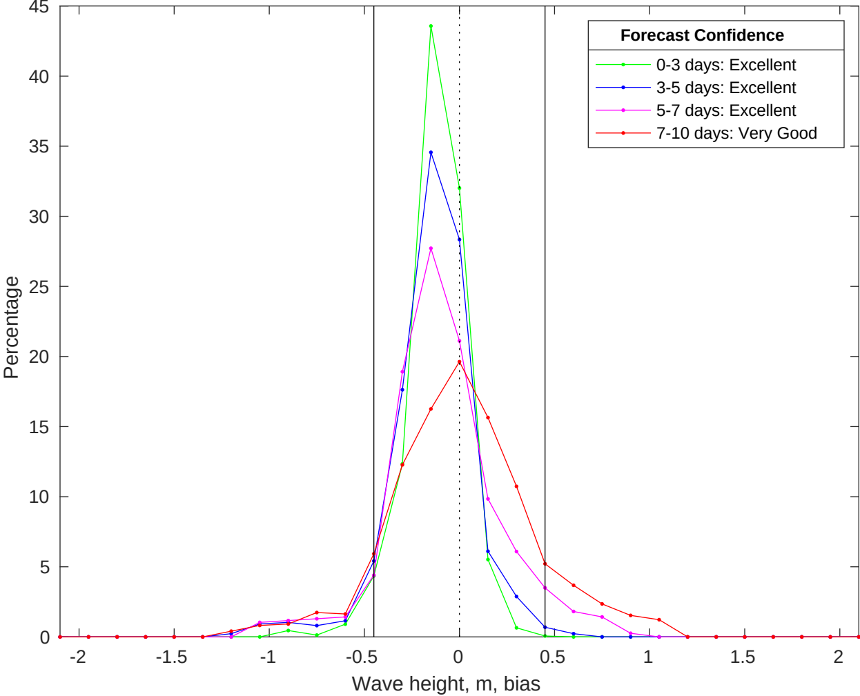
NDBC 42019 vs CMEMS Waves Bias Histogram: 18-Jun-2025
