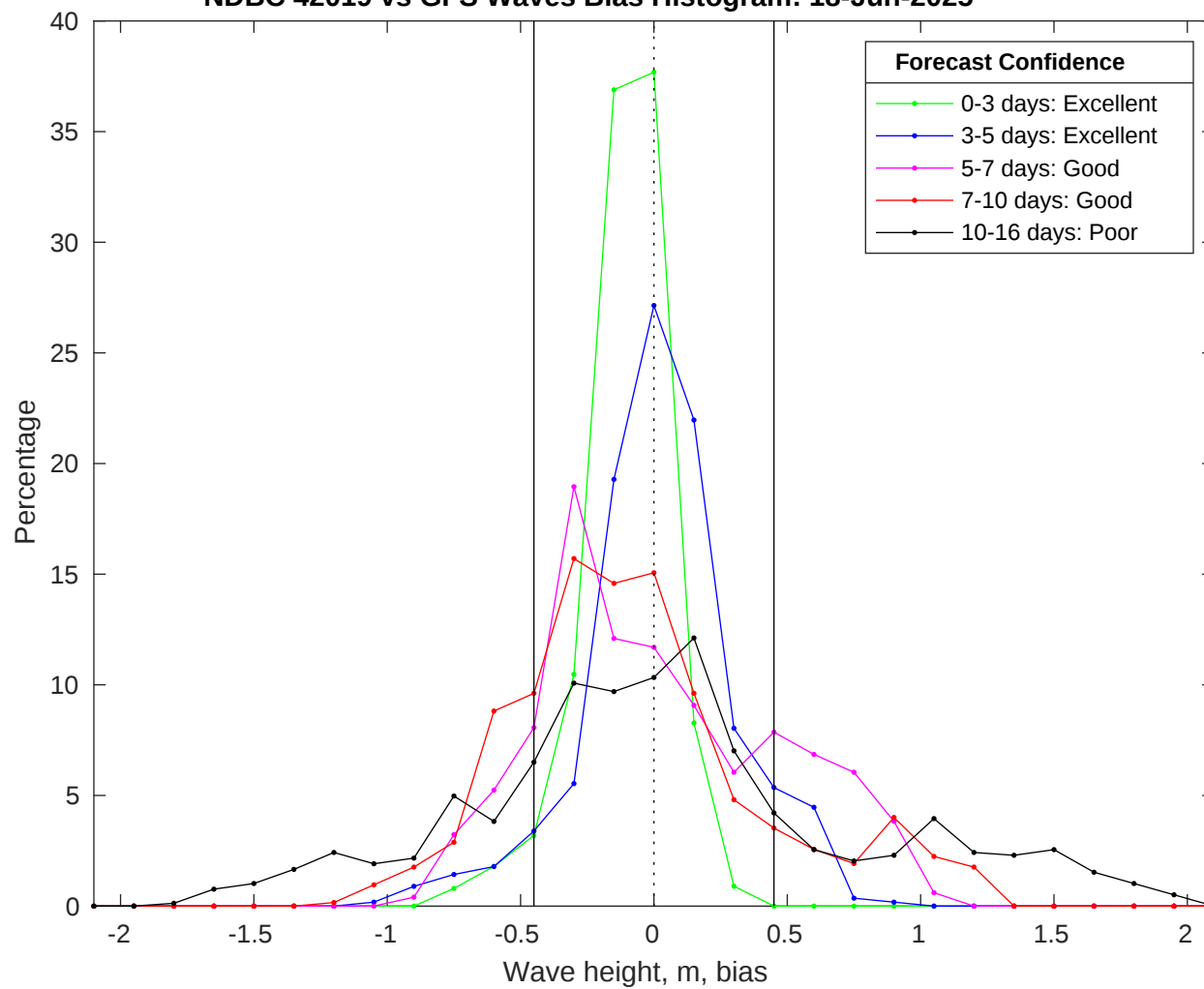
NDBC 42019 vs GFS Waves Bias Histogram: 18-Jun-2025
