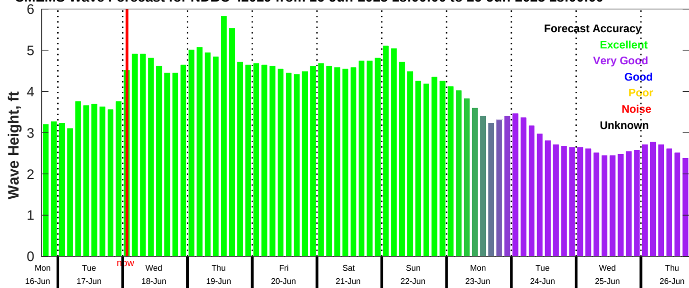
CMEMS Wave Forecast for NDBC 42019 from 16-Jun-2025 18:00:00 to 26-Jun-2025 18:00:00
