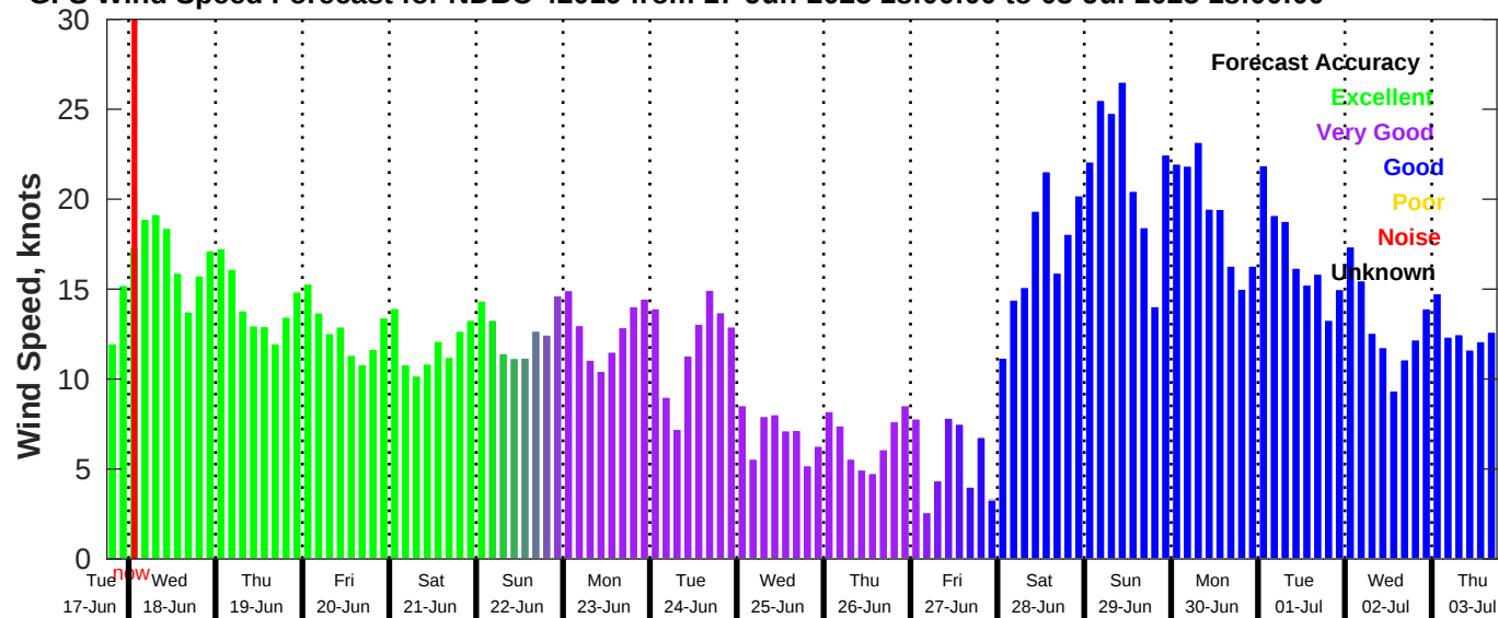
GFS Wind Speed Forecast for NDBC 42019 from 17-Jun-2025 18:00:00 to 03-Jul-2025 18:00:00
