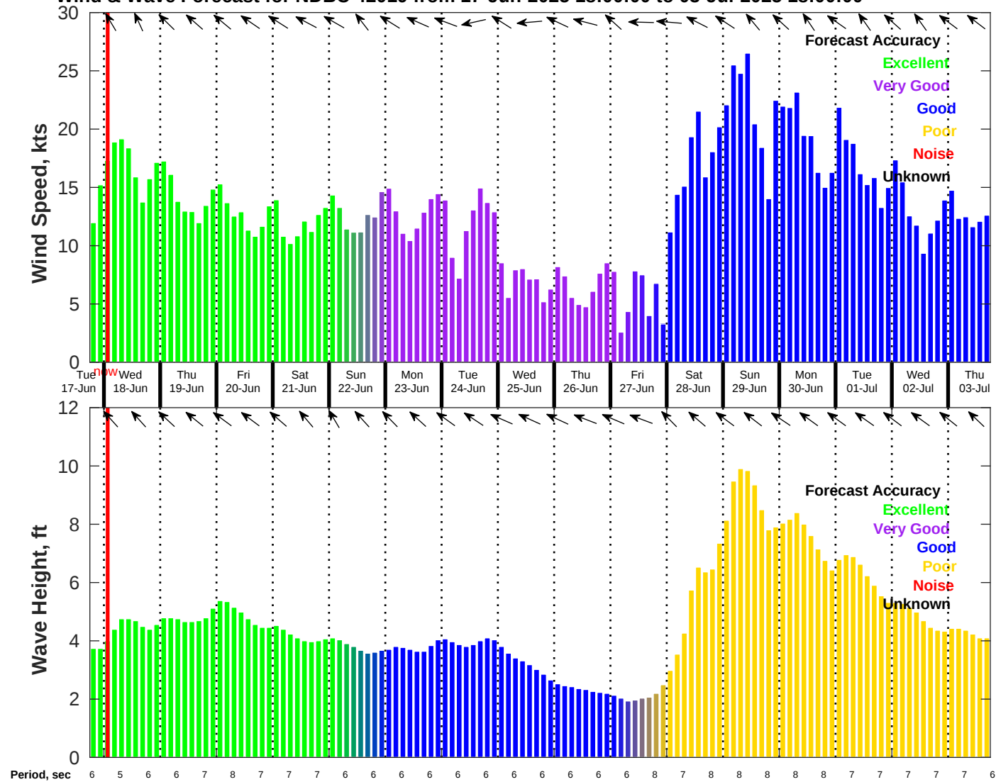
Wind & Wave Forecast for NDBC 42019 from 17-Jun-2025 18:00:00 to 03-Jul-2025 18:00:00
